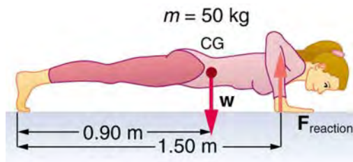
Figure 7.46 Forces involved in doing push-ups. The woman's weight acts as a force exerted downward on her center of gravity (CG).
