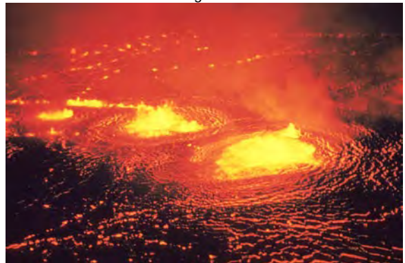
Figure 14.34 Lava flow on Kilauea volcano in Hawaii. (credit: J. P. Eaton, U.S. Geological Survey)
